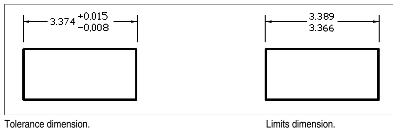
Tolerance dimension.
