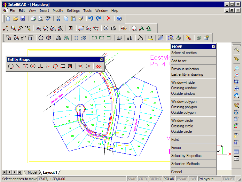
The IntelliCAD user interface.
